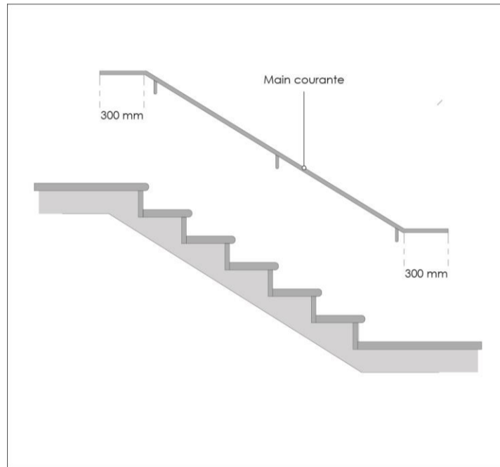
Illustration 5 Main courante
